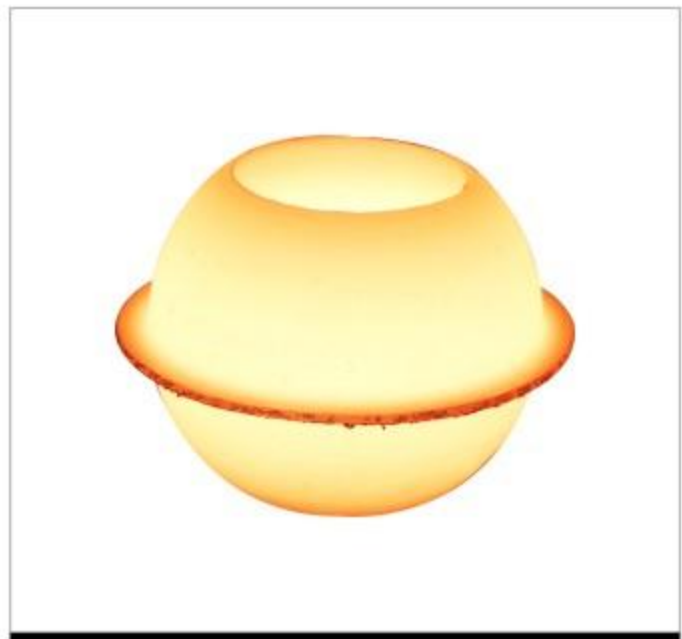
实心锻造球坯 Forged Solid Ball Blank
